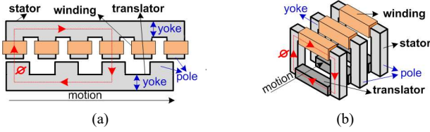
Fig. 1. Basic LSRM structure (a) LLSRM (b) TLSRM.
