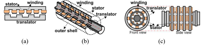
Fig. 3. LSRM (a) flat (D-1) (b) cylindrical (D-2) (c) rotary-linear (D-3).
